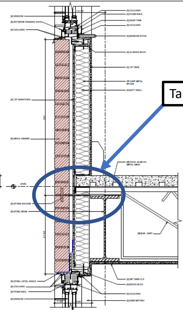
2 EXISTING WINDOW HEAD/SILL DETAIL 3" = 1'-0" Existing Brick Cladding
