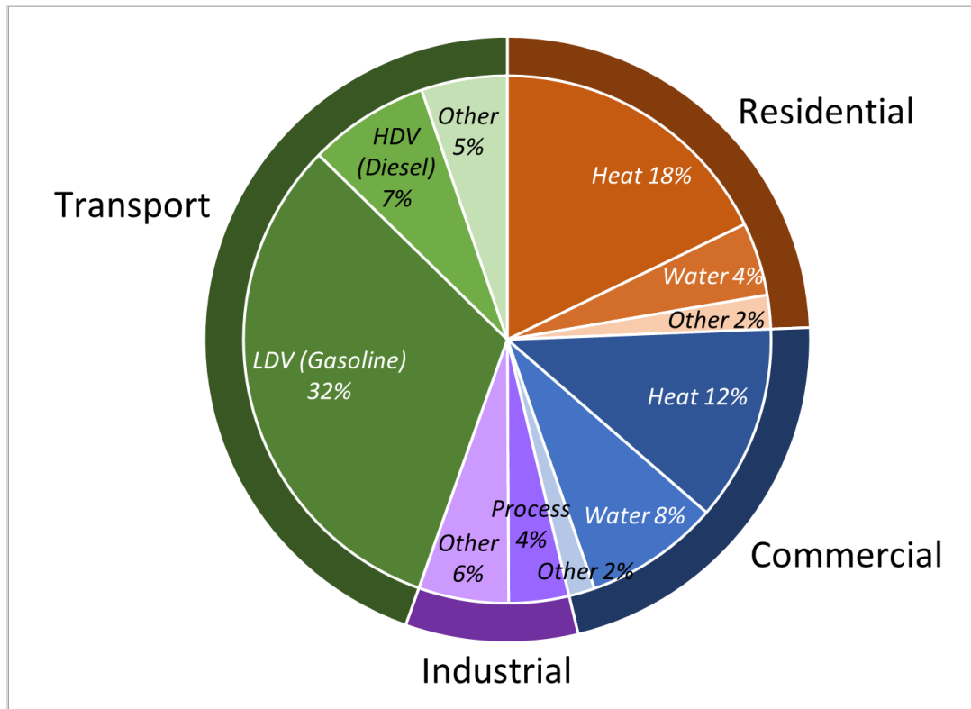
Figure 1: Direct fossil fuel use divided by end use and sector in New York and New England. The region uses about 4.2 quadrillion BTUs of direct fossil fuel energy each year.
