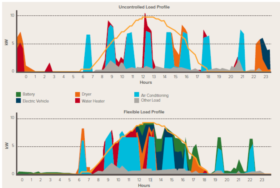
Figure 11: Impact of demand flexibility on residential load profile, from RMI 2018
