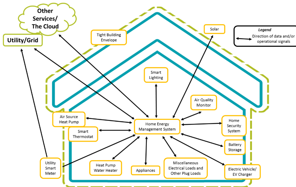
ES Figure 2: The Decarbonized Smart Energy Home of the Future
